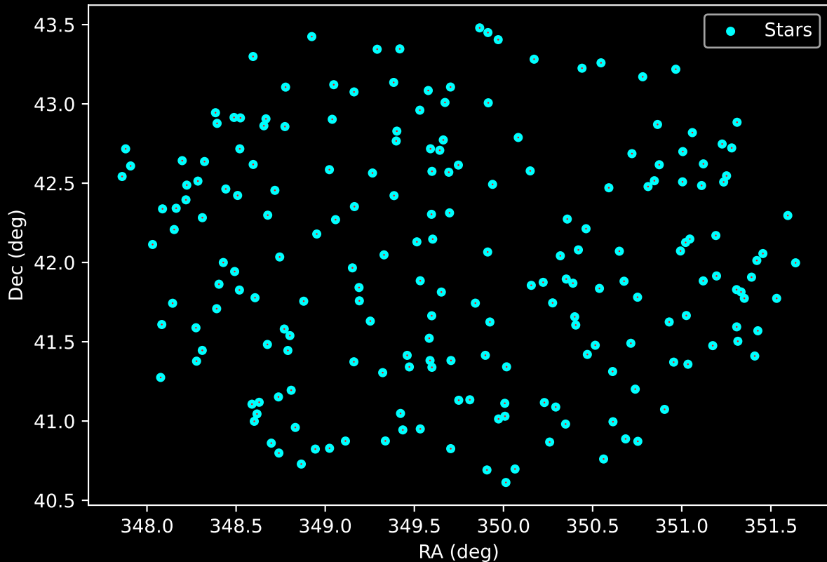
APOGEE DR17 Field: [066+42_MGA] Proper Motion Vectors for Gaia Star Field (n= 203)
