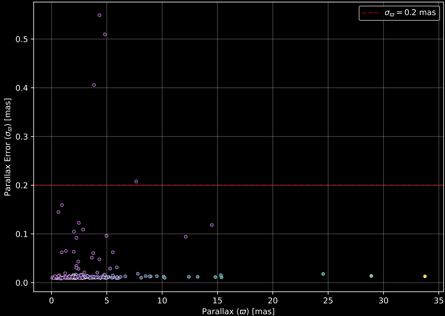
APOGEE DR17 Field: [066+42_MGA] Parallax Quality (n= 203)
