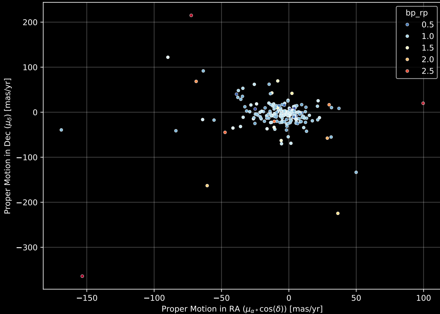
APOGEE DR17 Field: [066+42_MGA] Proper Motion Diagram (n= 203)
