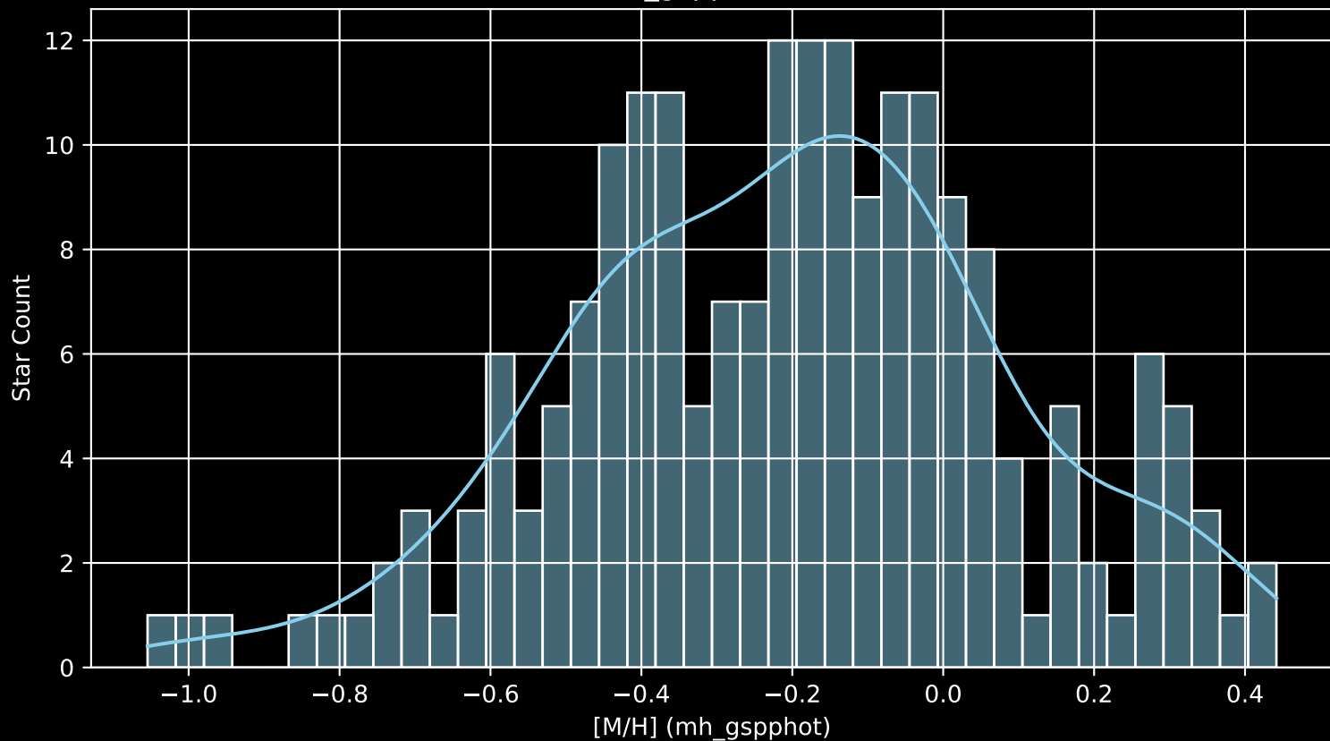
APOGEE DR17 Field: [066+42_MGA [M/H] (mh_gspphot) (n= 201)
