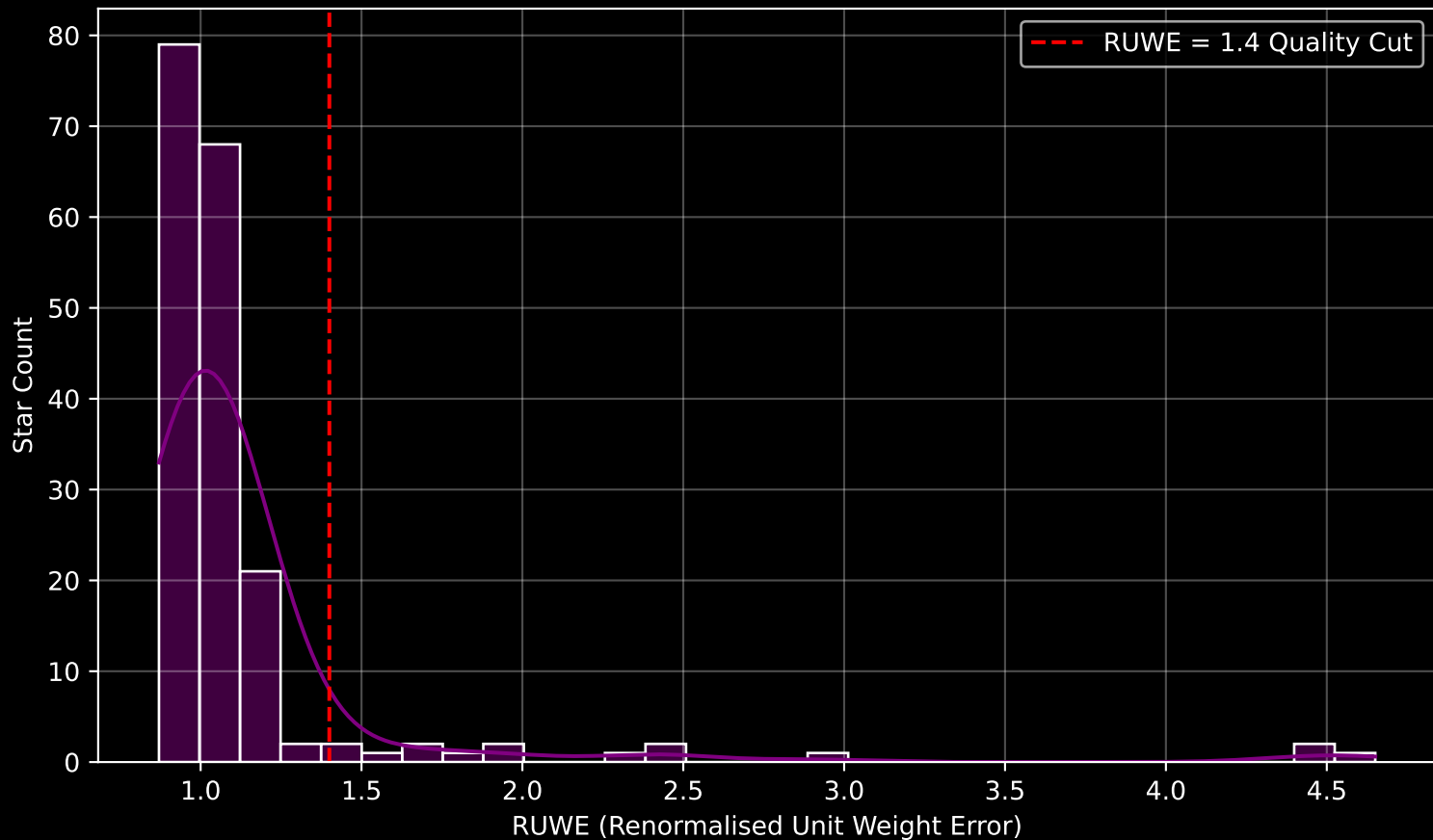
GAPOGEE DR17 Field [066+42_MGA] RUWE Distribution (n= 185)
