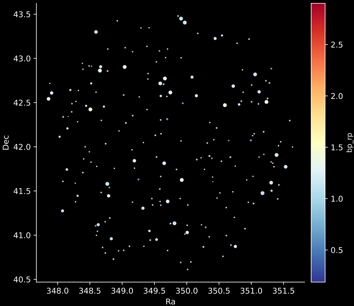
APOGEE DR17 Field: [066+42_MGA] Stars: 203
