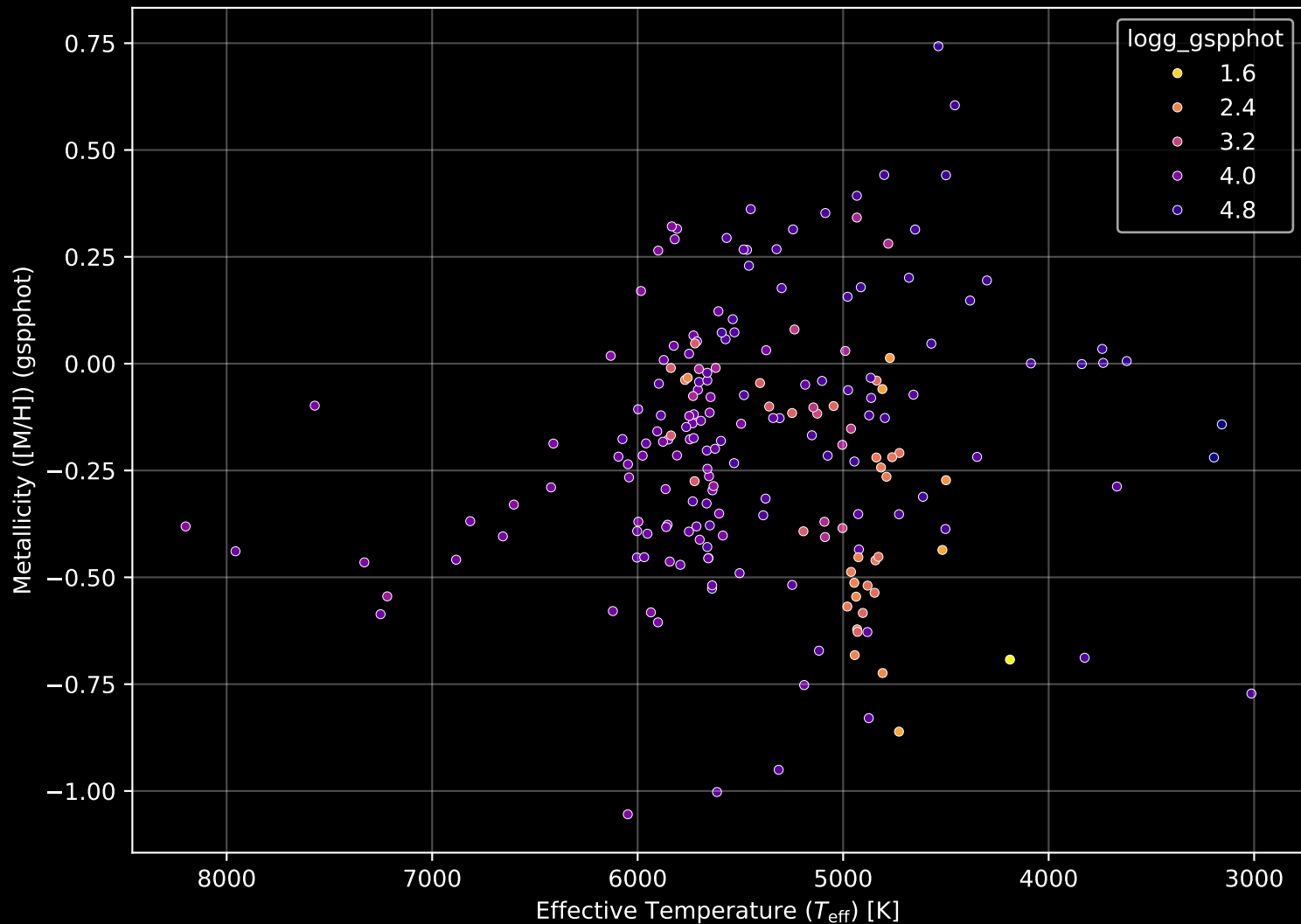
APOGEE DR17 Field: [066+42_MGA] Stellar Population Parameters (n= 203)
