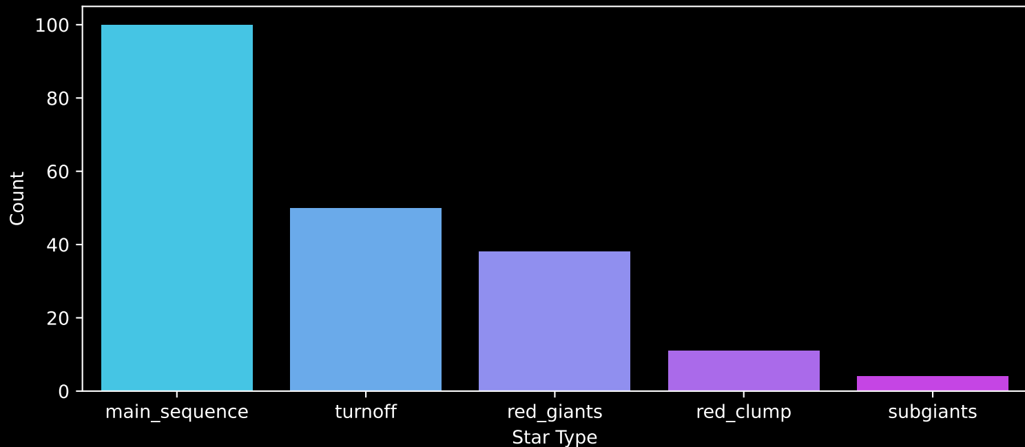
APOGEE DR17 Field: [066+42_MGA] Count plot of Star Type
